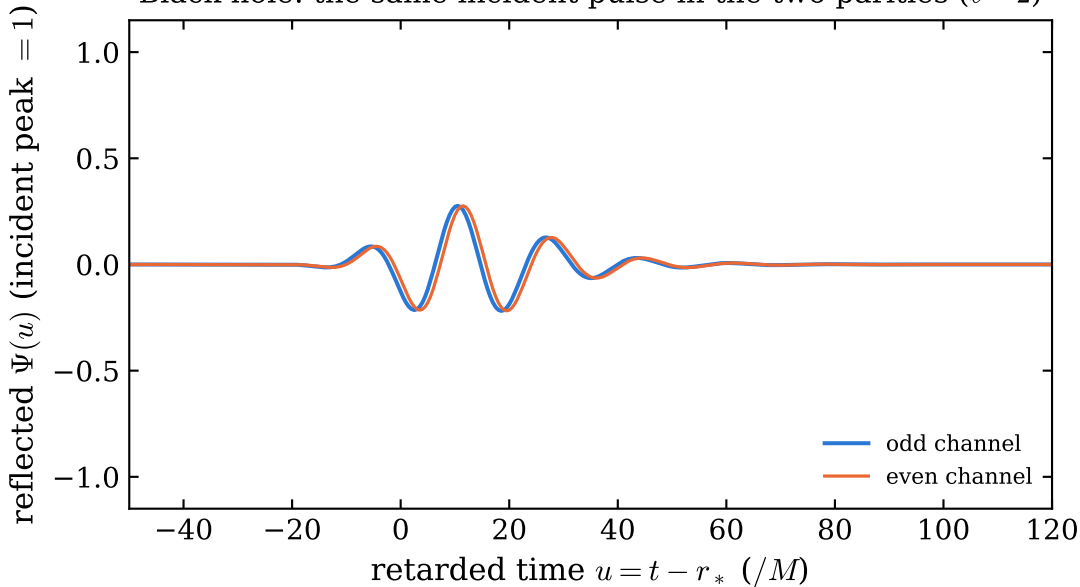
Black hole: the same incident pulse in the two parities ( \ell = 2 )
